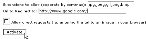
Figure 4.86: Enabling hotlink protection
