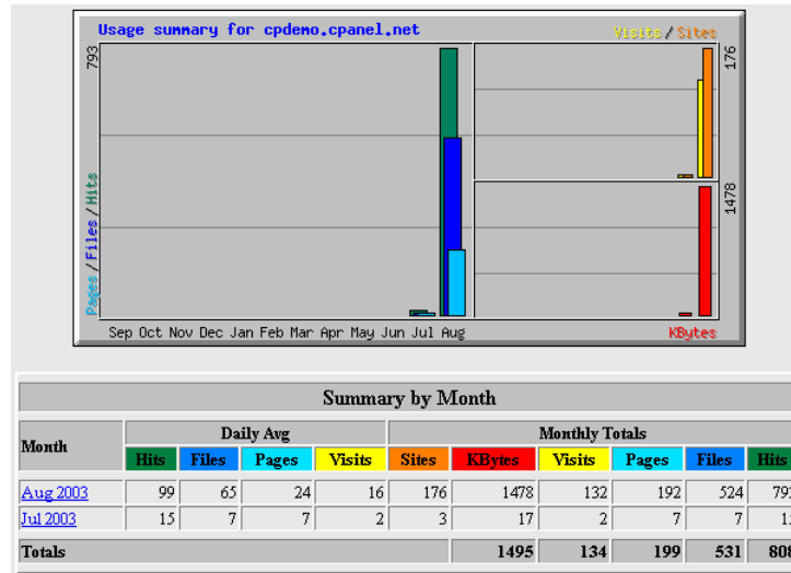
Figure 4.61: Webalizer statistics
