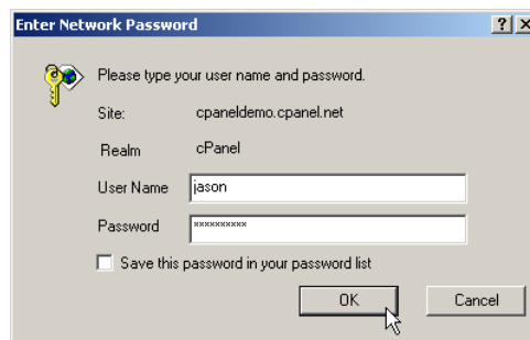
Figure 4.1: Logging on
